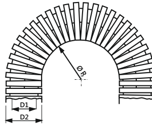
DIMENSION DRAWING & TECHNICAL DETAILS
