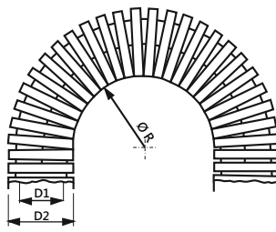
DIMENSION DRAWING & TECHNICAL DETAILS
