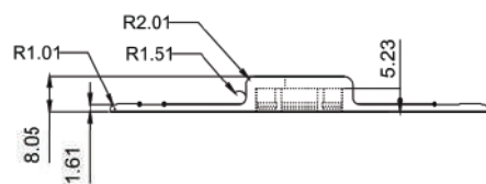
ROUND BASE FOR DC CLIP
