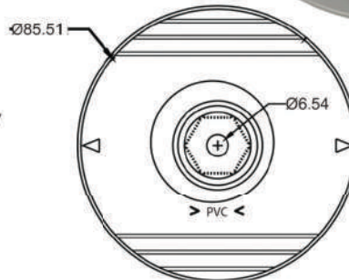
M6X12 CSK SCREW
