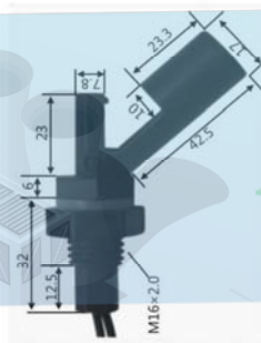
FS-43 FLOAT SWITCHES
