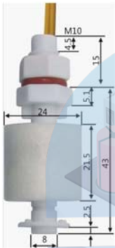
FS-43 FLOAT SWITCHES
