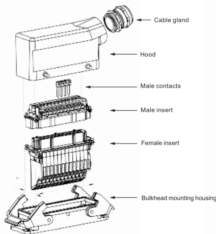
⑤ Through-panel connector and side entry type.
