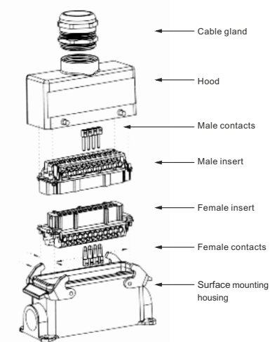
④ Surface mounting and top entry type.
