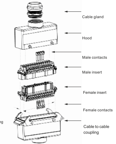
⑥ Cable to cable and top entry type.
