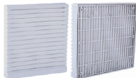
ETAV-05 SIZE: 238mm x 238mm(Screw Fit) Colour shade: RAL-7032/7035 Std. Packing : 60 Nos.
