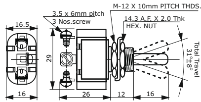
SINGLE POLE UNSEALED
