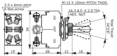
DOUBLE POLE UNSEALED
