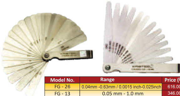
Feeler Gauge - 26 Blades | 13 Blades
